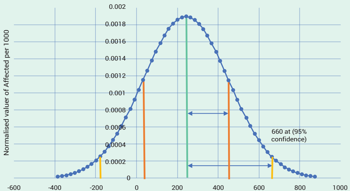
Figure 4.1: Normal distribution curve of affected population (2014-2020)
